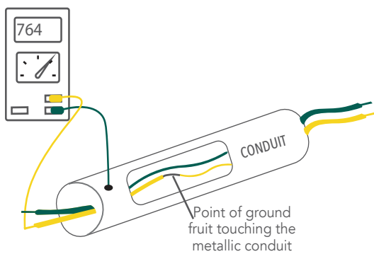
Figure 138: Continuity test
