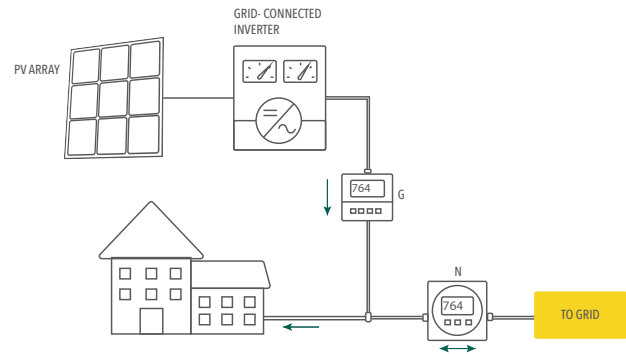
Figure 66: Grid-Connected Inverter
