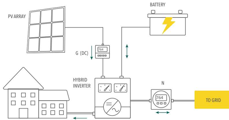
Figure 68: Hybrid Inverter
