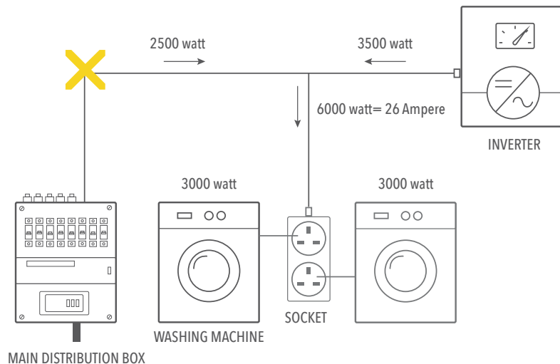
Figure 75: Wrong connection from main distribution box at customer’s residence
