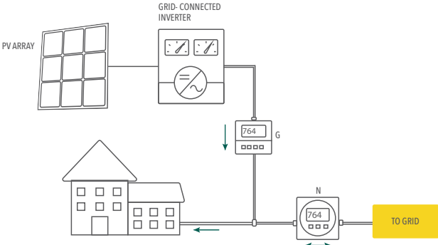
Figure 3: Grid connected PV System
