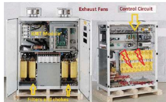
Figure 70: Central inverter internal structure
