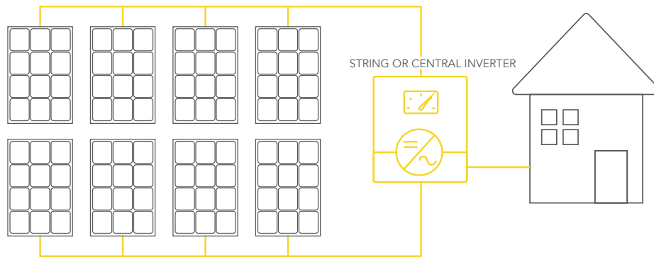
Figure 71: String Inverter
